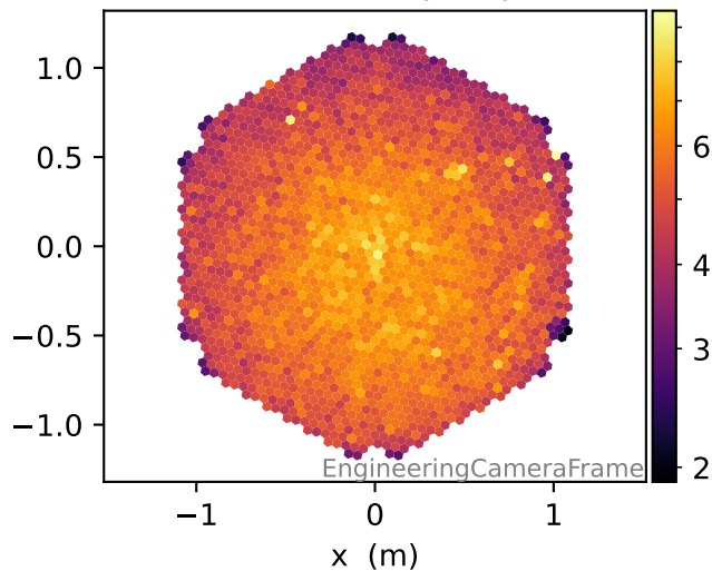
Fraction of >1000 p.e. pulses
