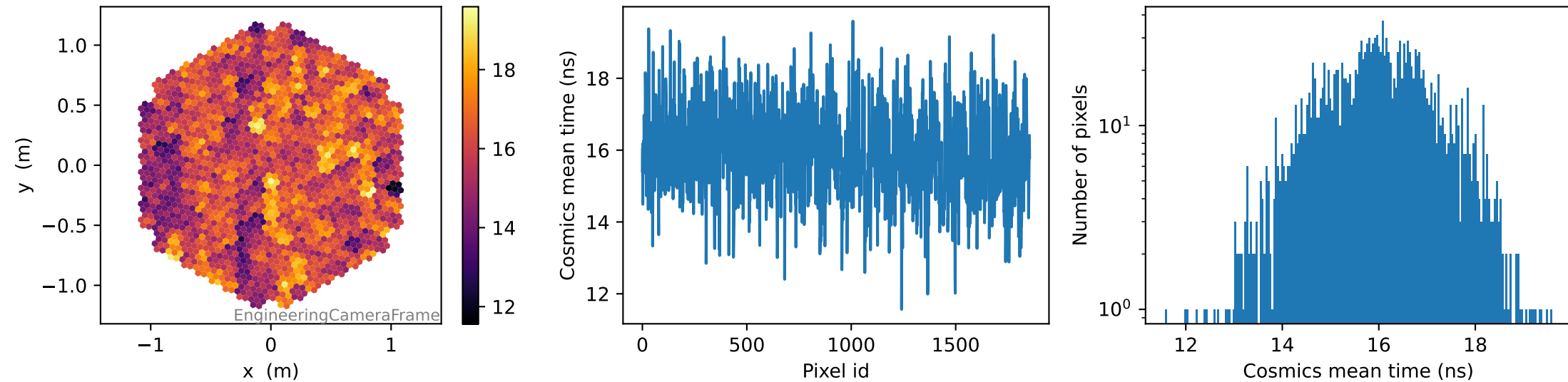
Cosmics mean time (ns)
