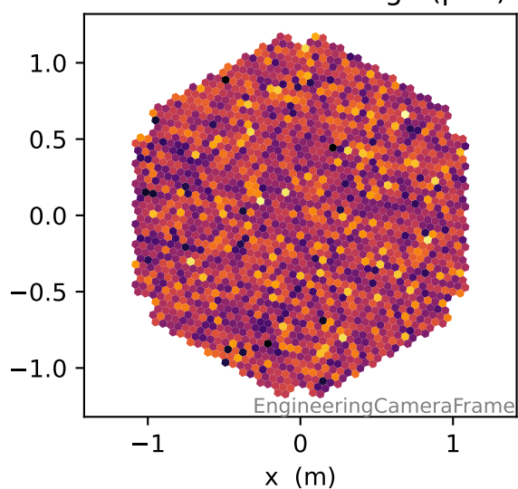
Flat-field charge std dev (p.e.)
