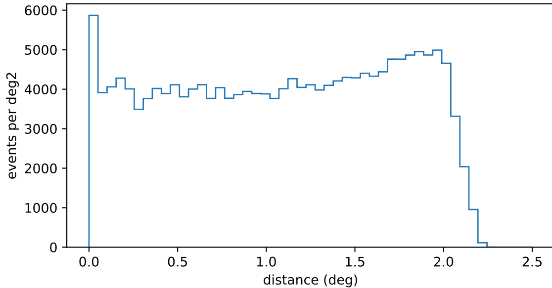
cog radial distribution, intensity > 200p
