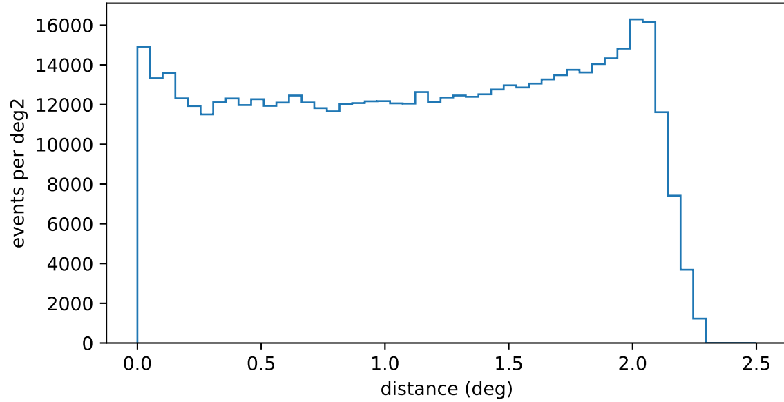
cog radial distribution, intensity > 200p
