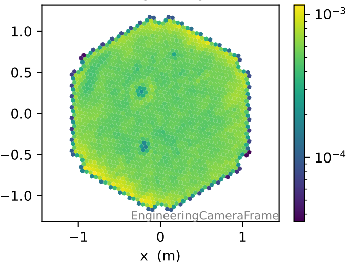
Image c.o.g., intensity > 200pe
