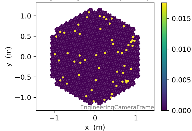
Image c.o.g., intensity > 200\text{pe}
