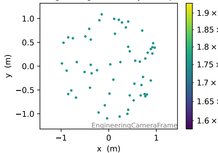
Image c.o.g., intensity > 200\text{pe}
