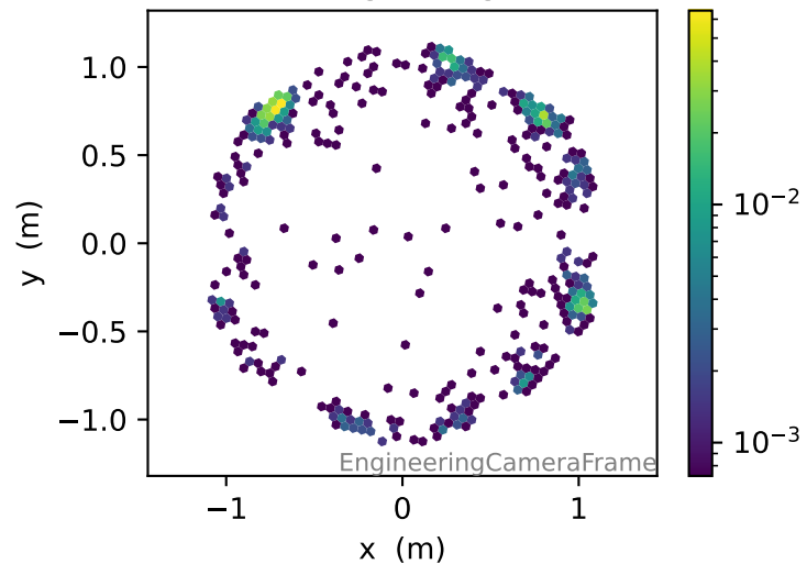
Image c.o.g., intensity > 200\text{pe}
