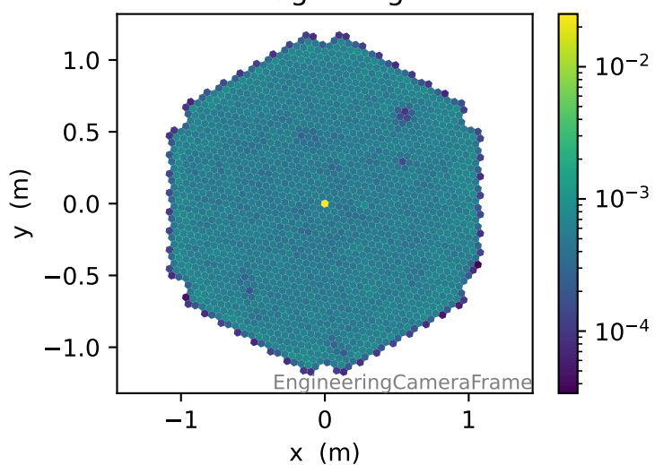
Image c.o.g., intensity > 200pe
