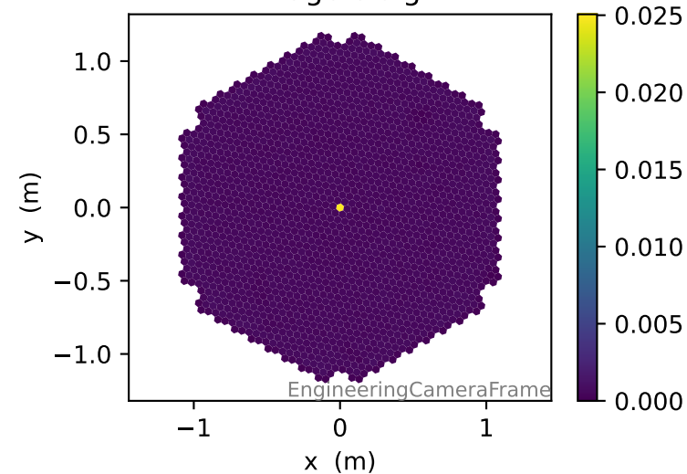
Image c.o.g., intensity > 200pe
