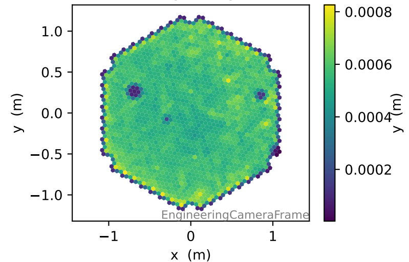
Image c.o.g., intensity > 200pe
