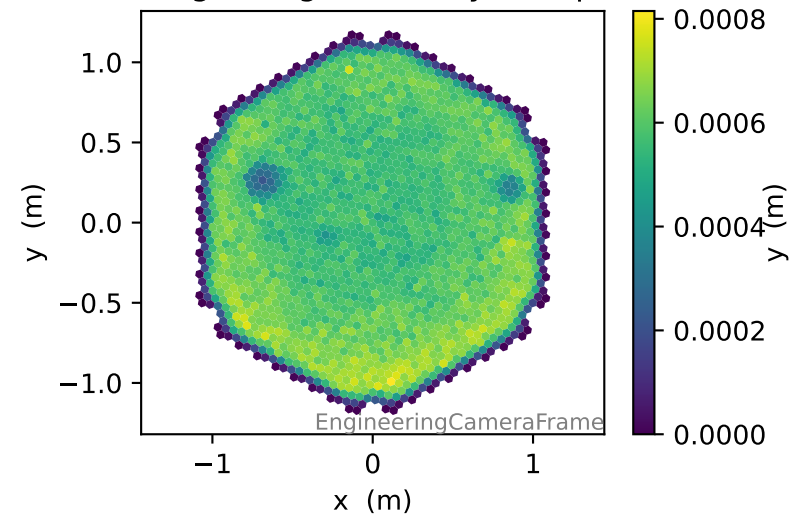
Image c.o.g., intensity > 200pe
