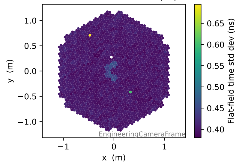
Flat-field time std dev (ns)
