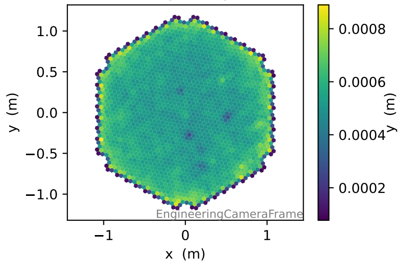
Image c.o.g., intensity > 200pe
