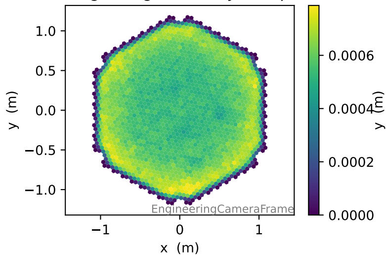
Image c.o.g., intensity > 200pe
