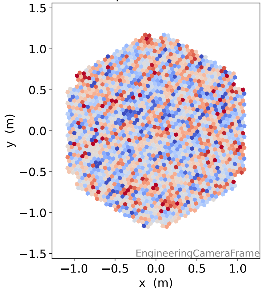
LG pedestal std [ADC]
