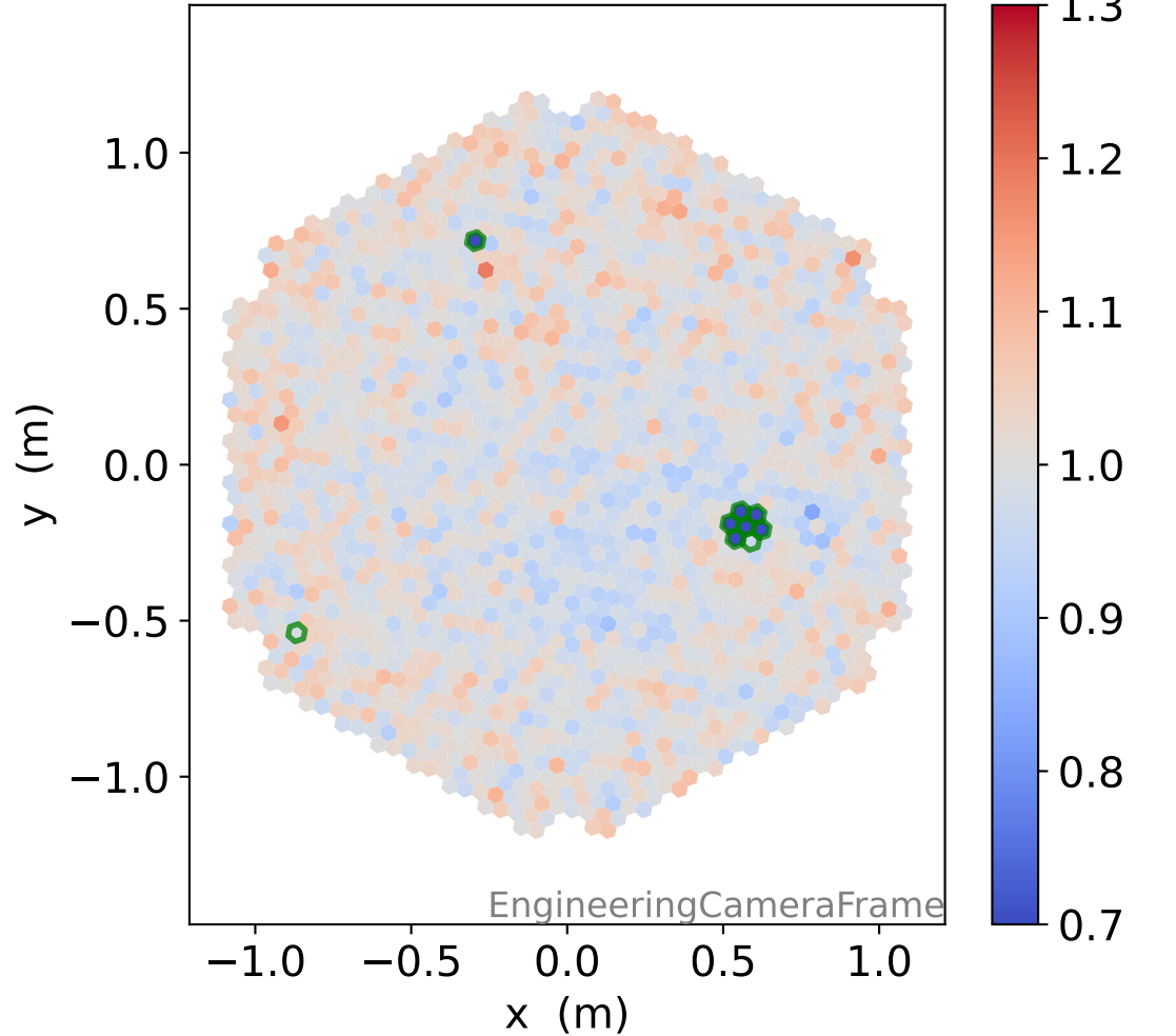
LG photon-electrons
