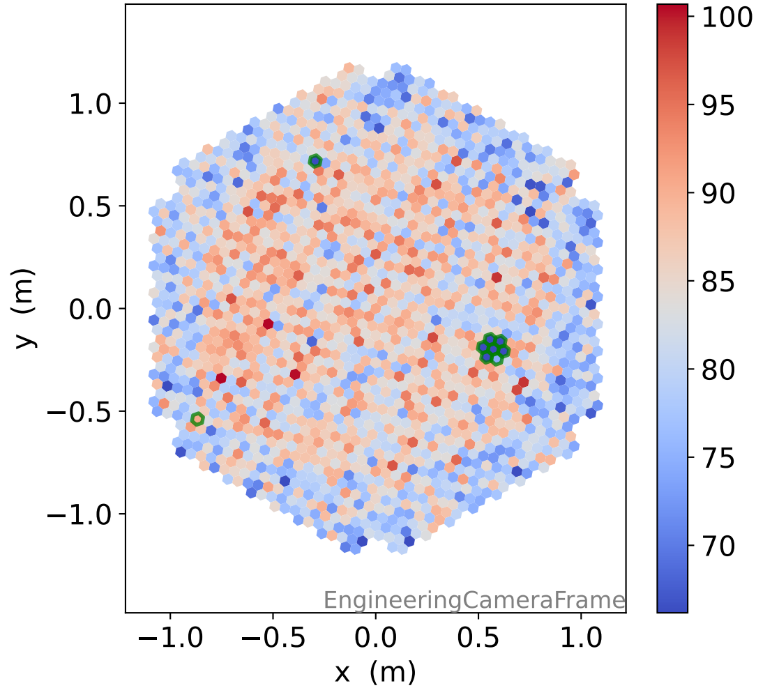
LG photon-electrons
