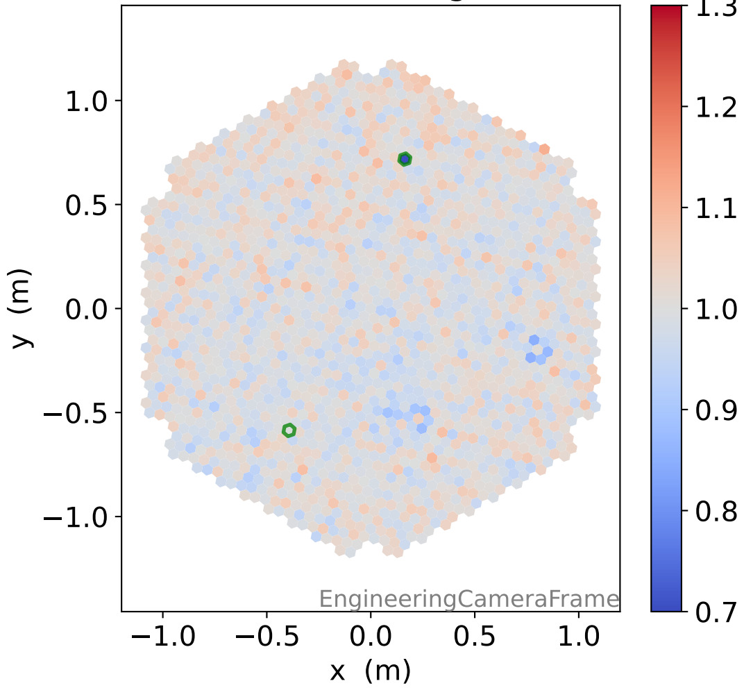
HG photon-electrons
