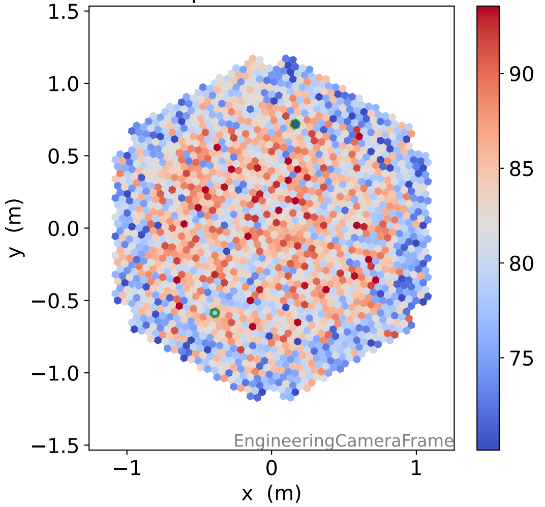
HG photon-electrons
