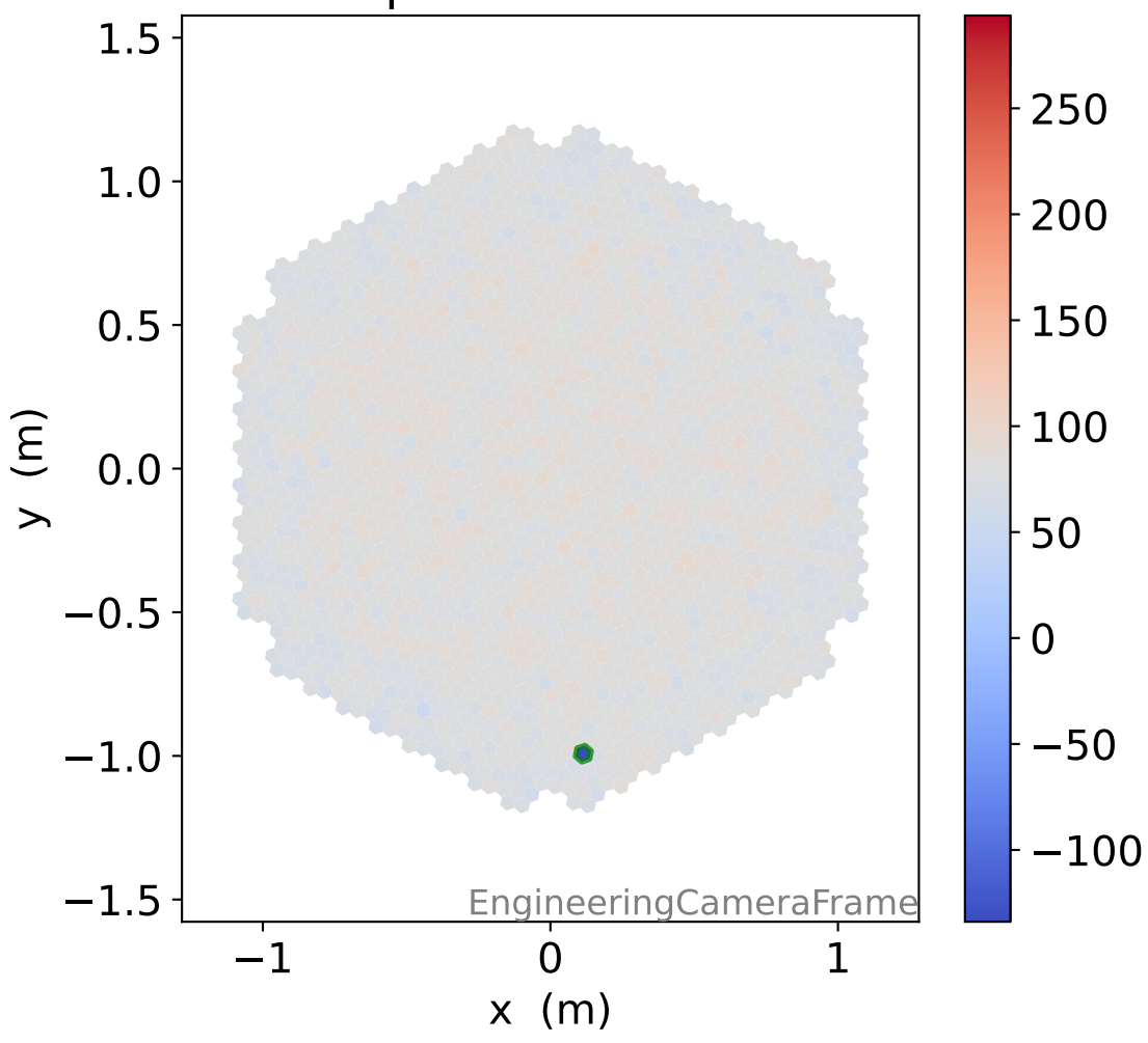
HG photon-electrons
