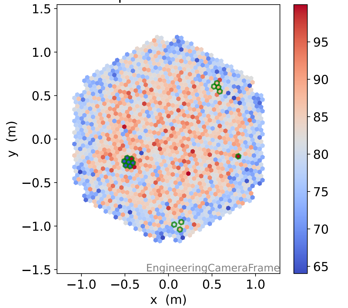
LG photon-electrons
