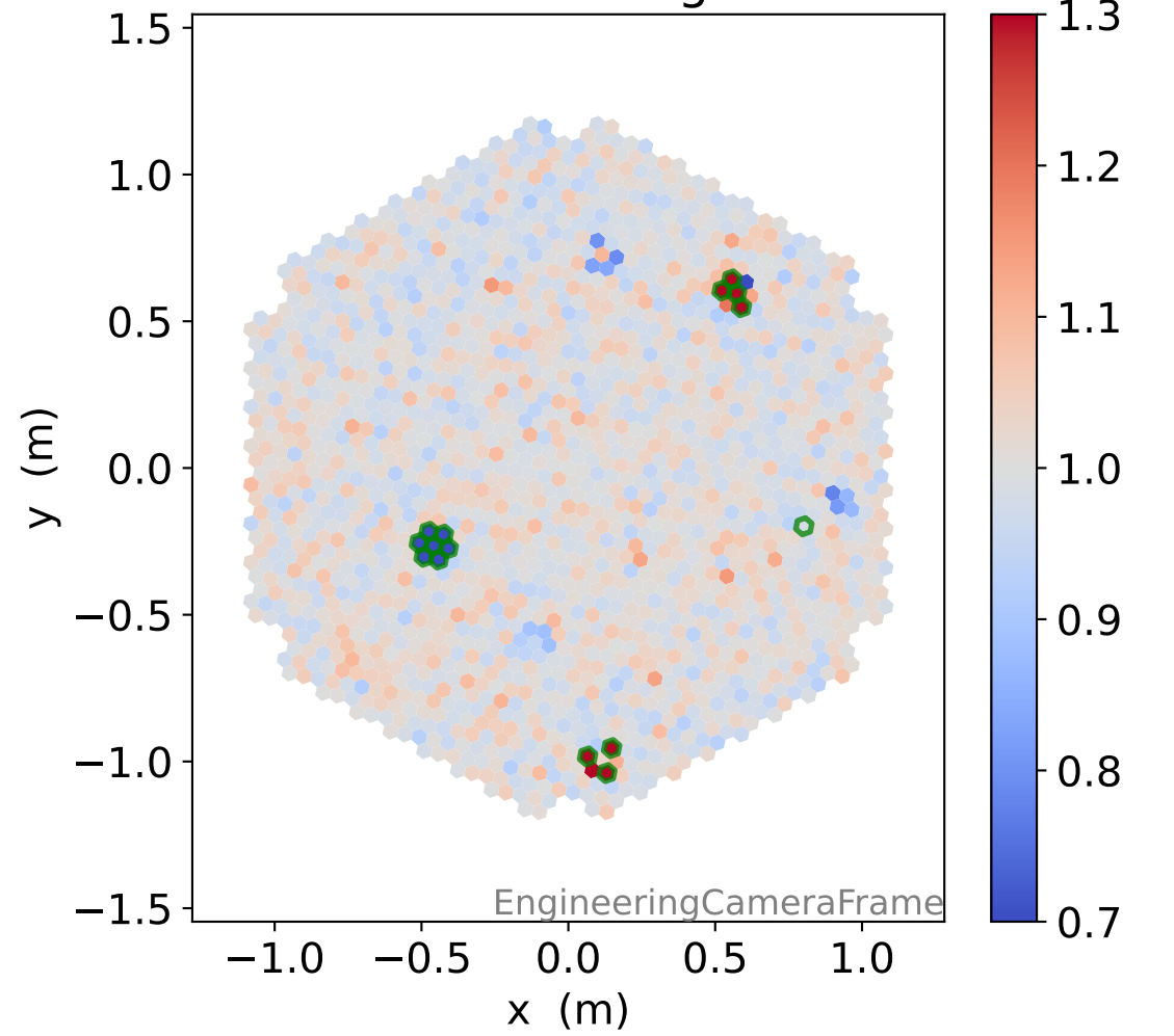
LG photon-electrons
