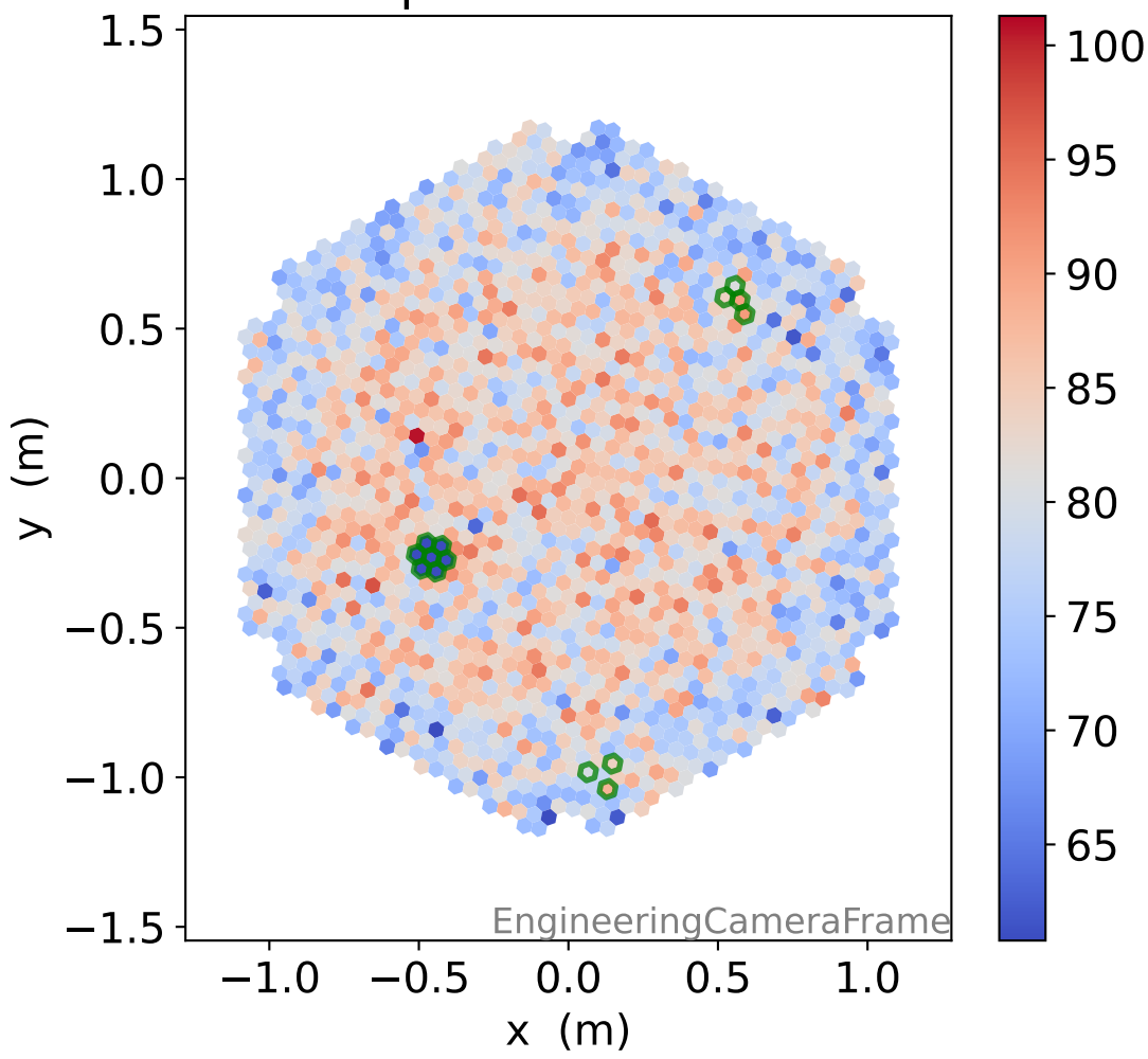
HG photon-electrons
