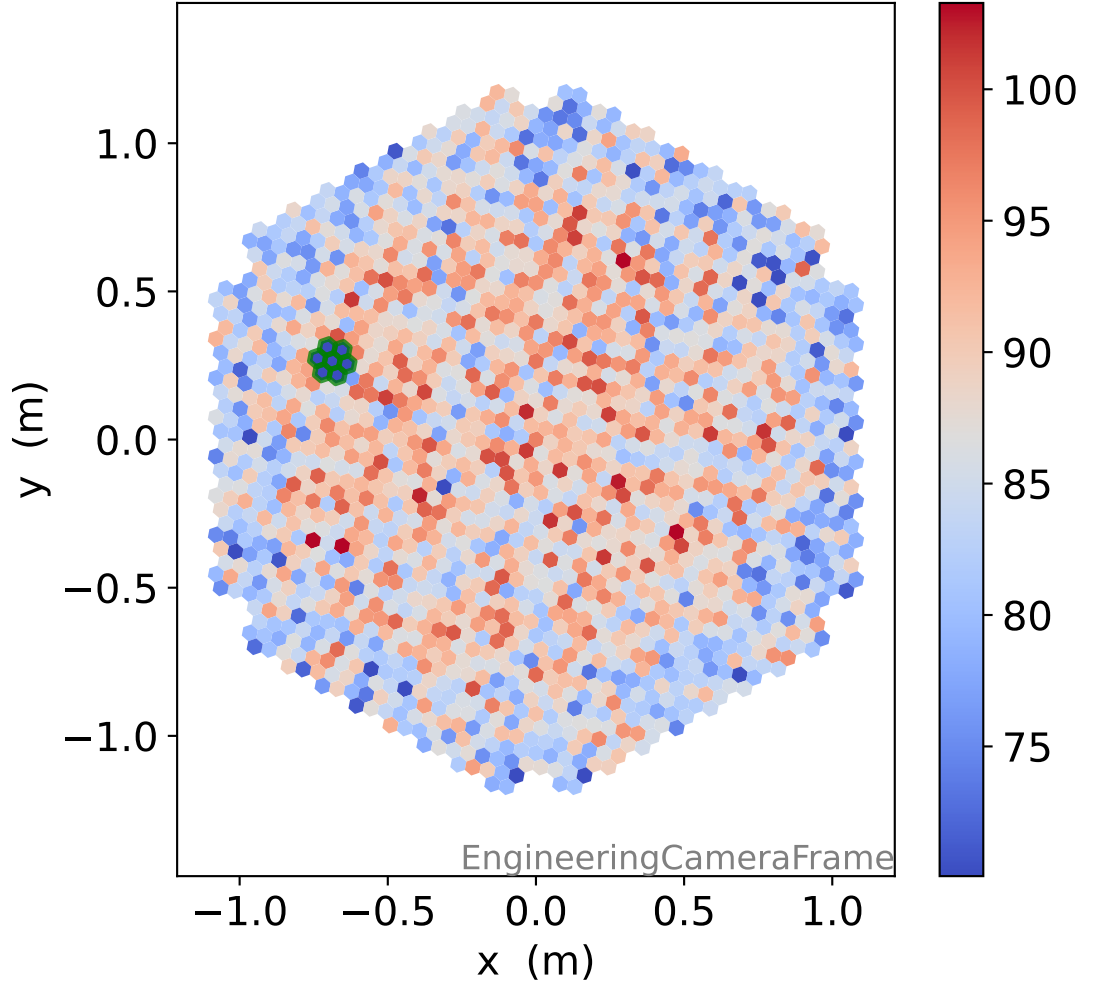
HG photon-electrons
