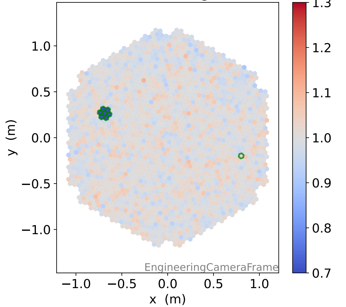
LG photon-electrons
