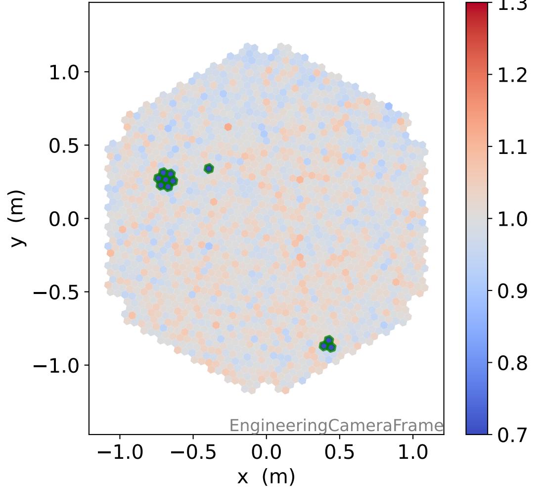
LG photon-electrons
