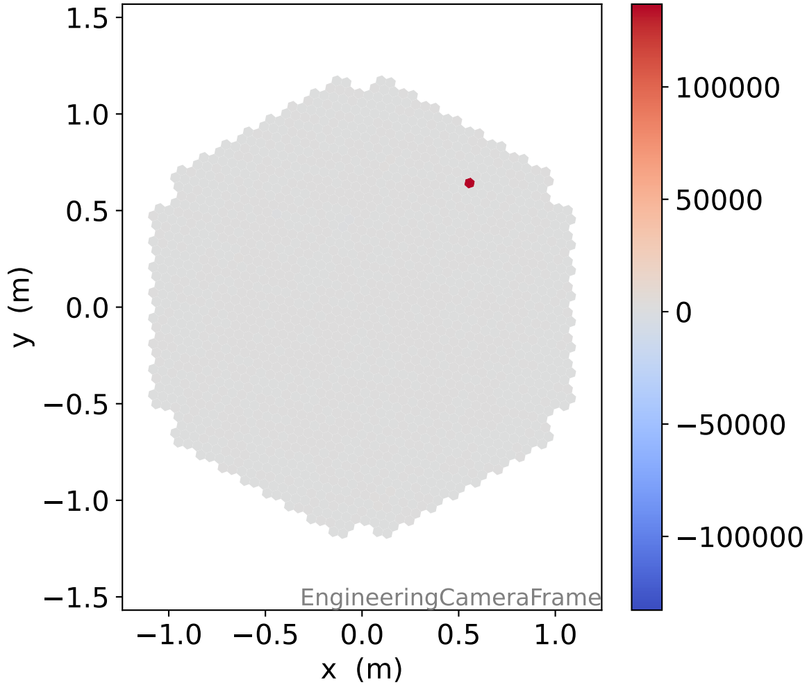
LG photon-electrons
