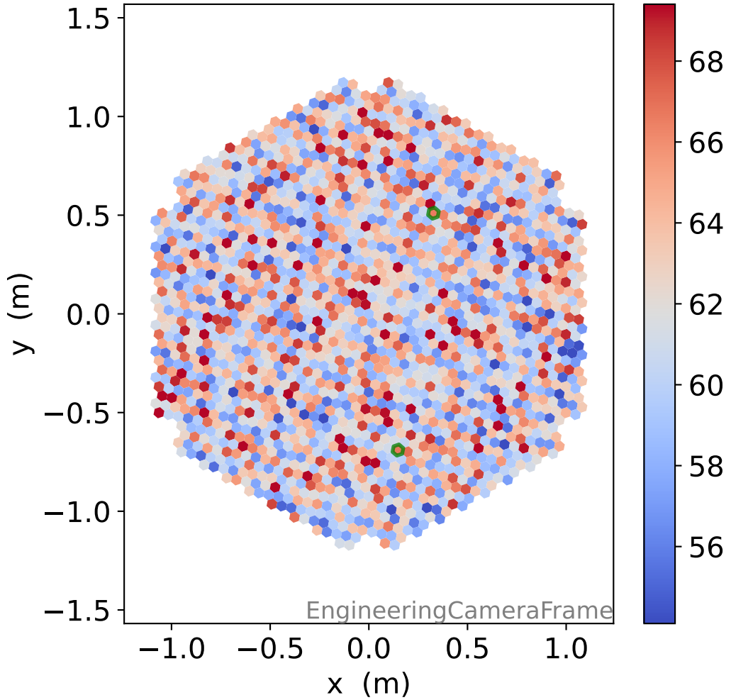
HG photon-electrons
