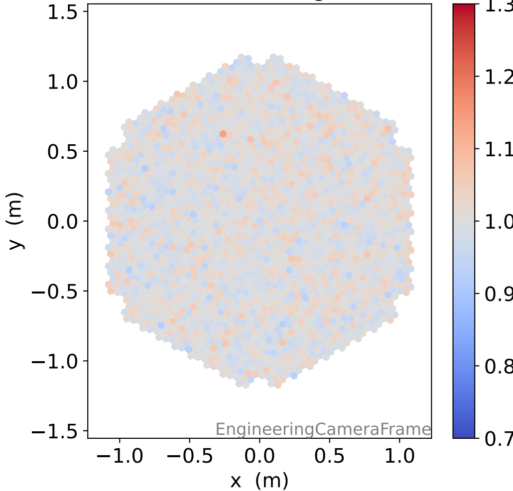
LG photon-electrons
