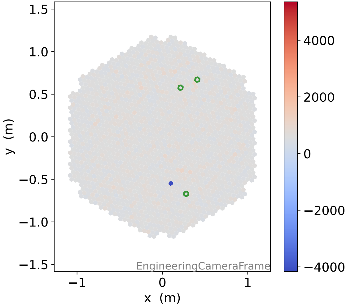
HG photon-electrons
