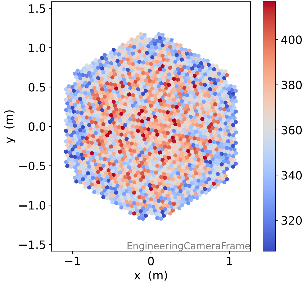
LG photon-electrons
