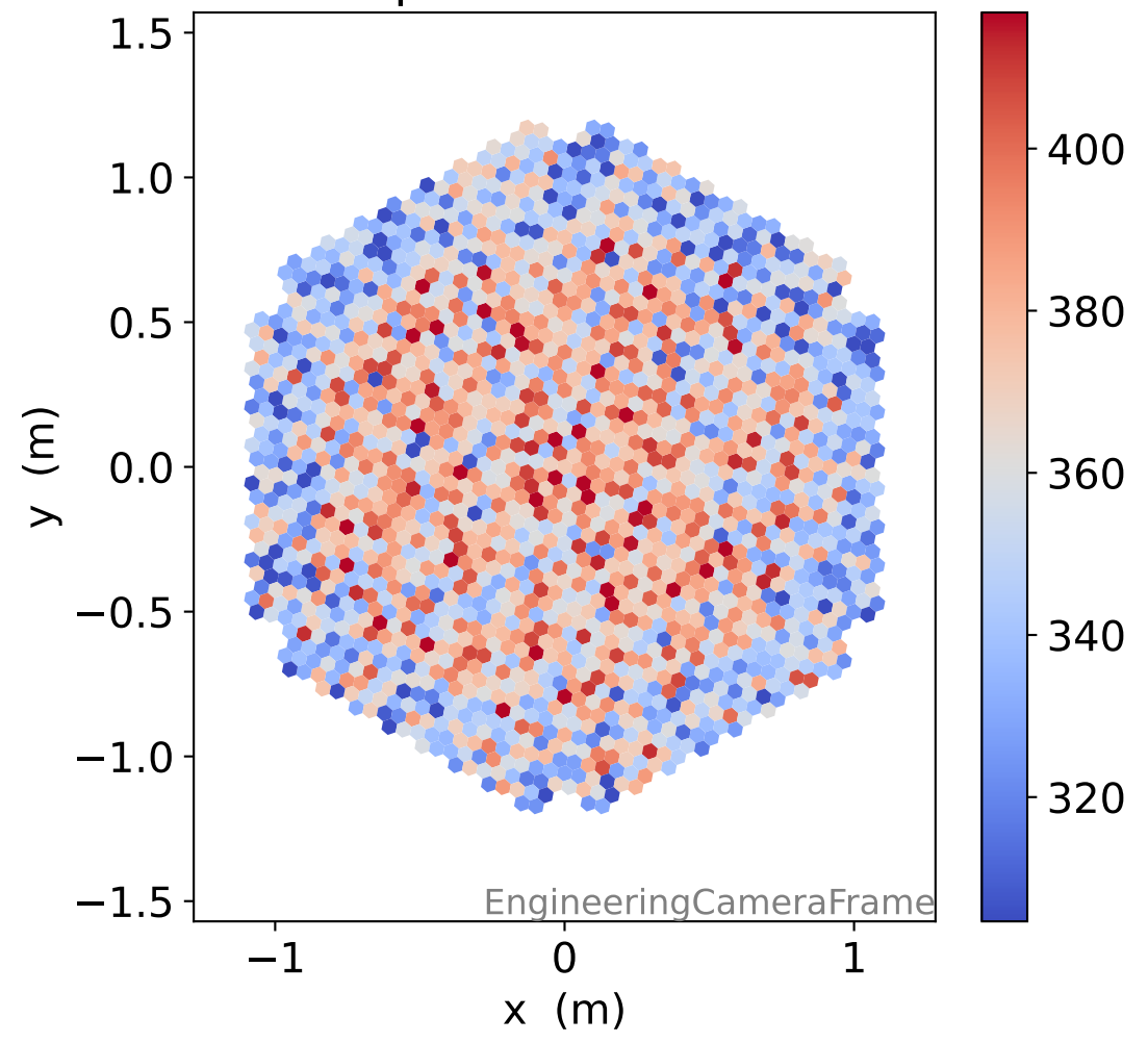
LG photon-electrons
