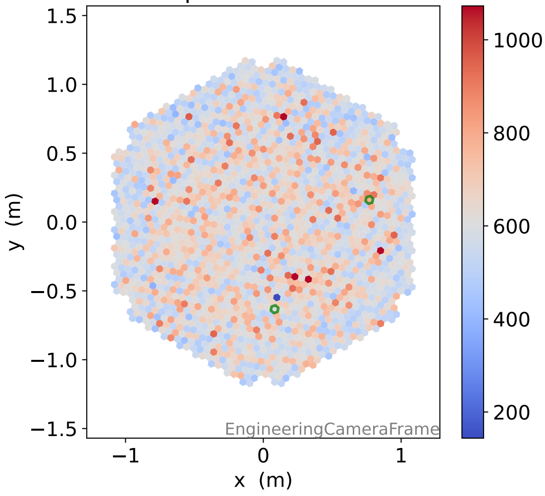
HG photon-electrons
