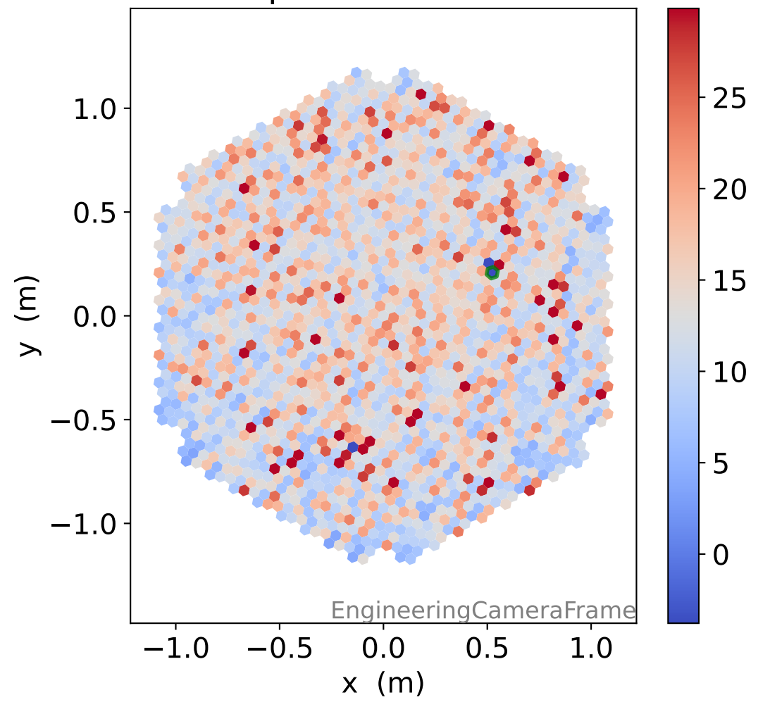
LG photon-electrons
