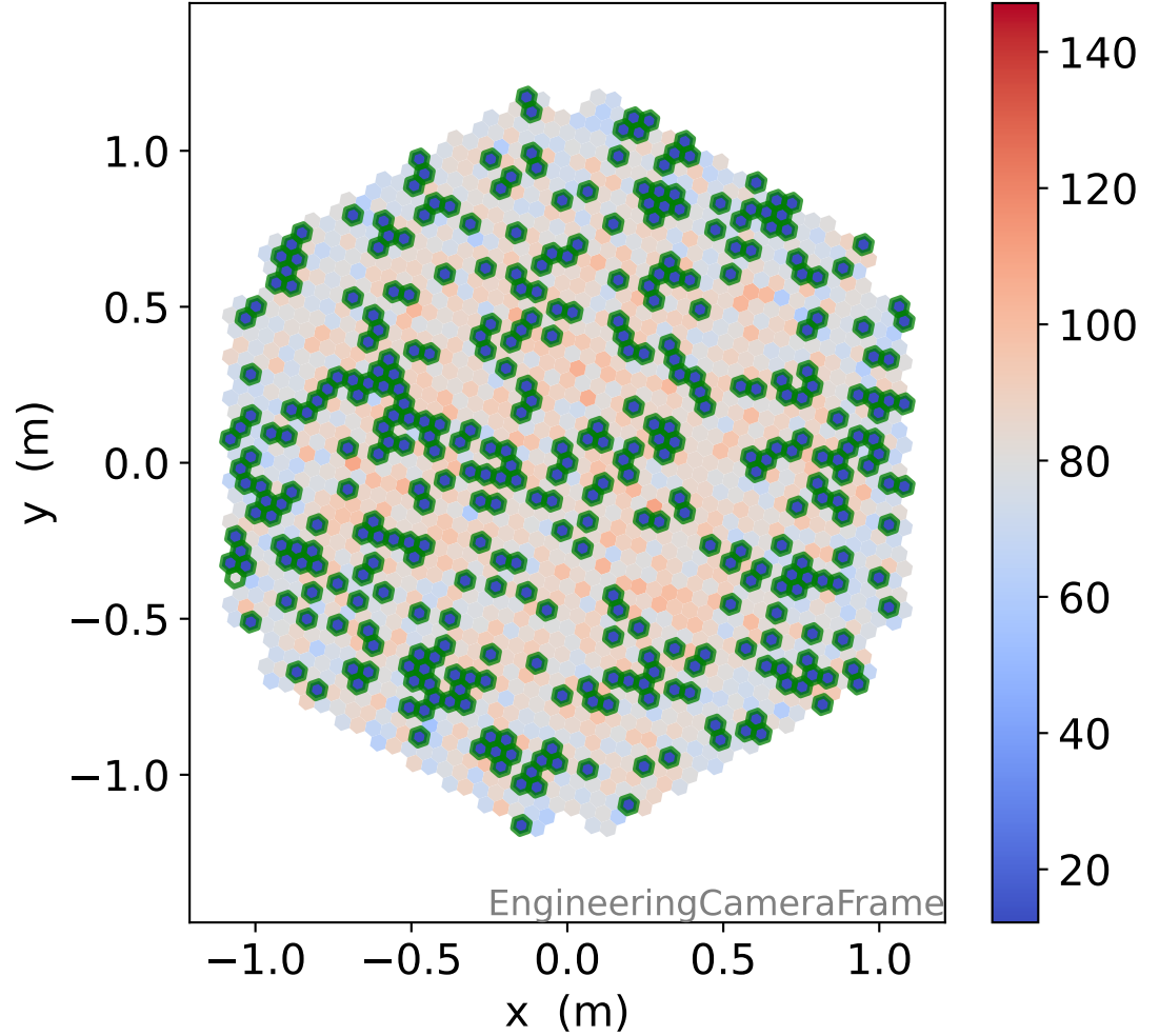
HG photon-electrons
