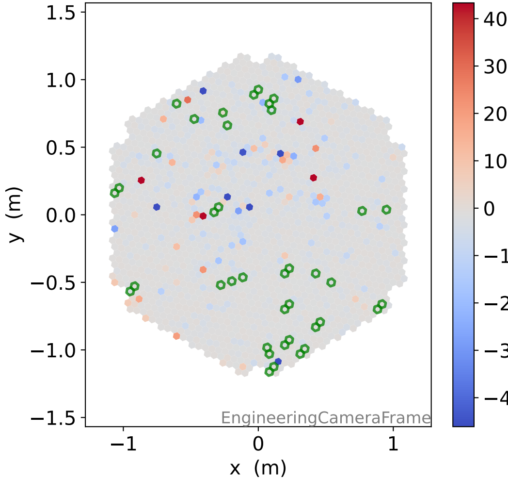
LG photon-electrons
