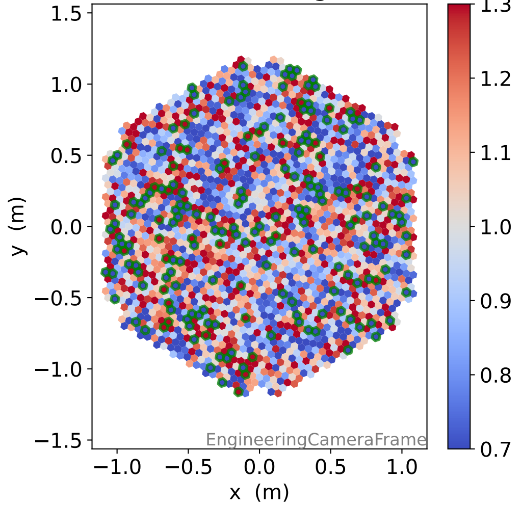
LG photon-electrons
