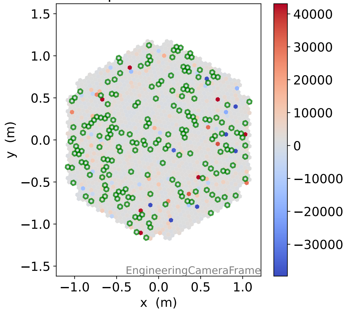
LG photon-electrons
