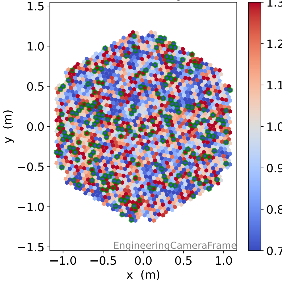
HG photon-electrons
