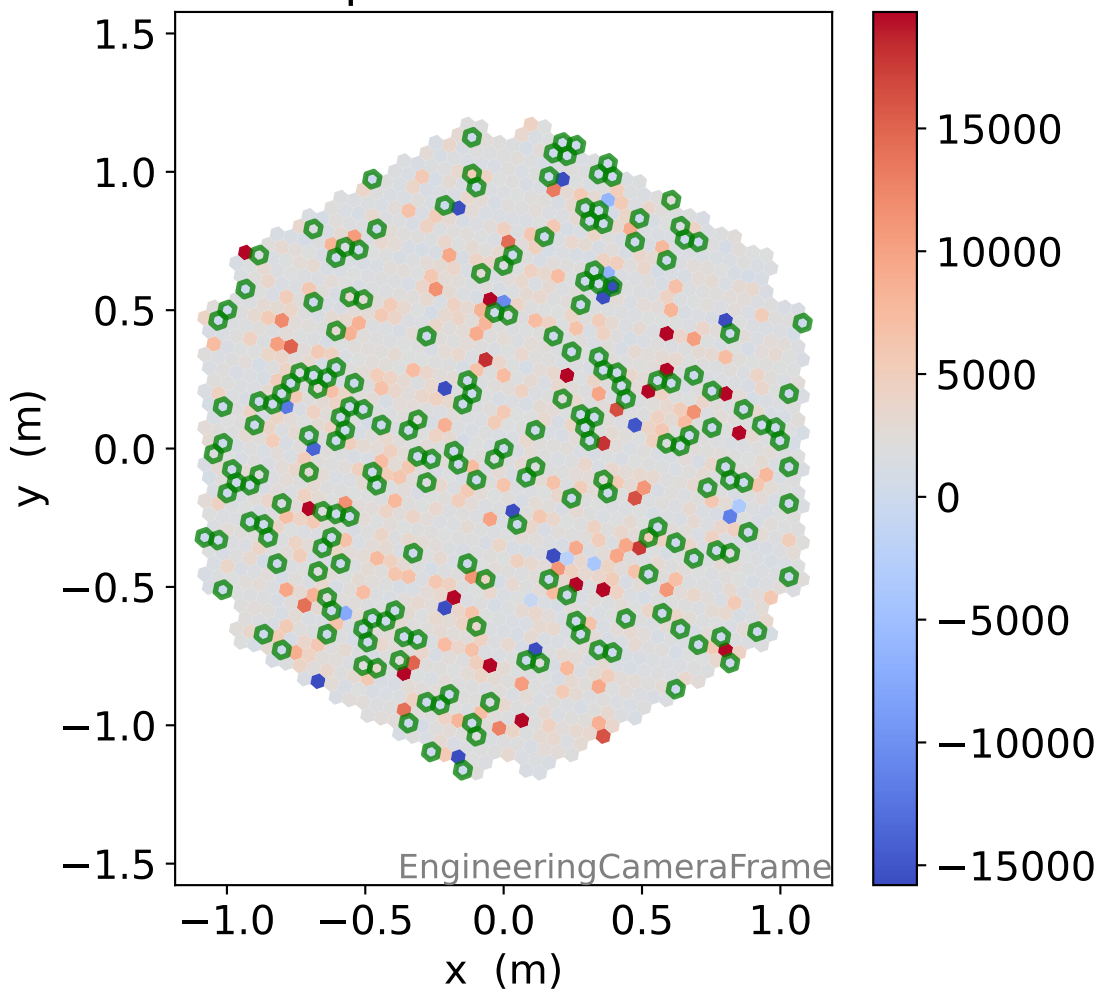
HG photon-electrons
