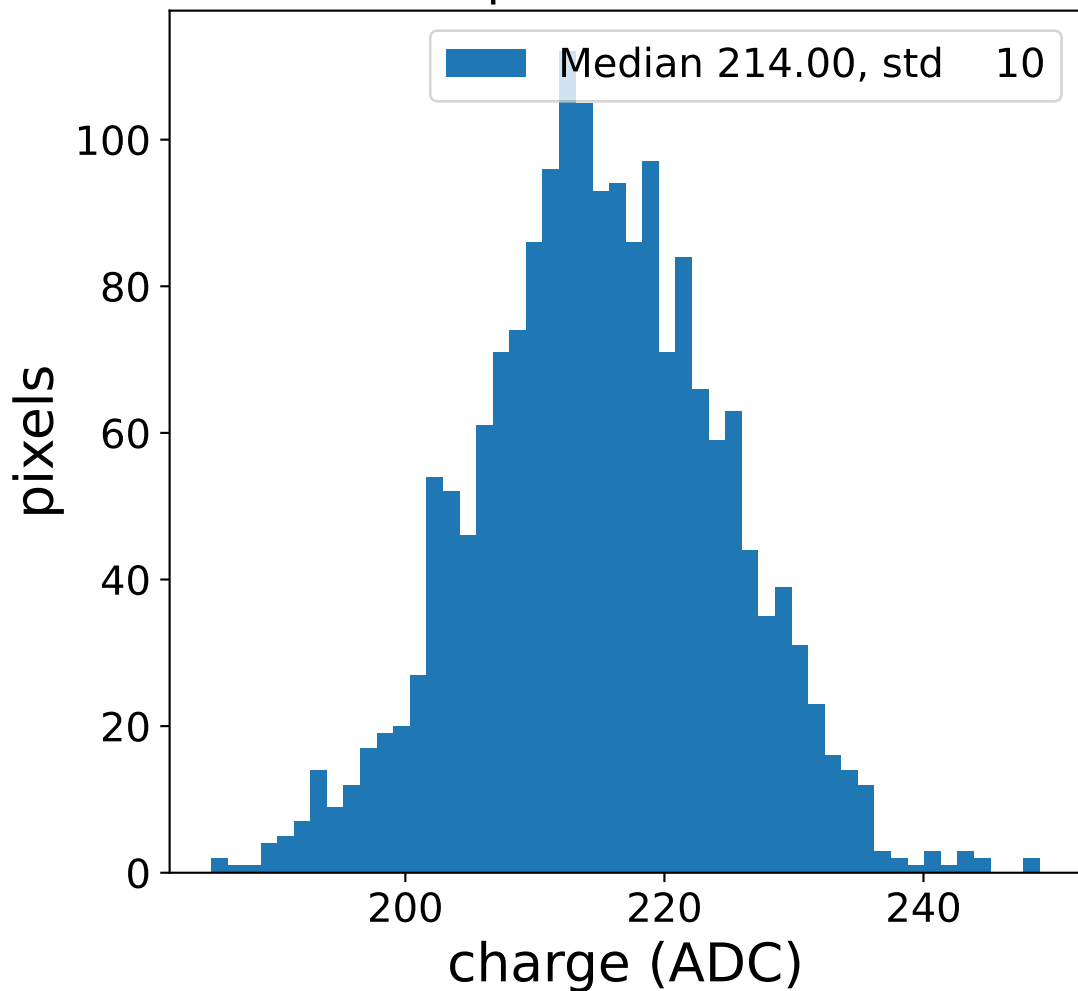
pedestal sample of 5096 events
