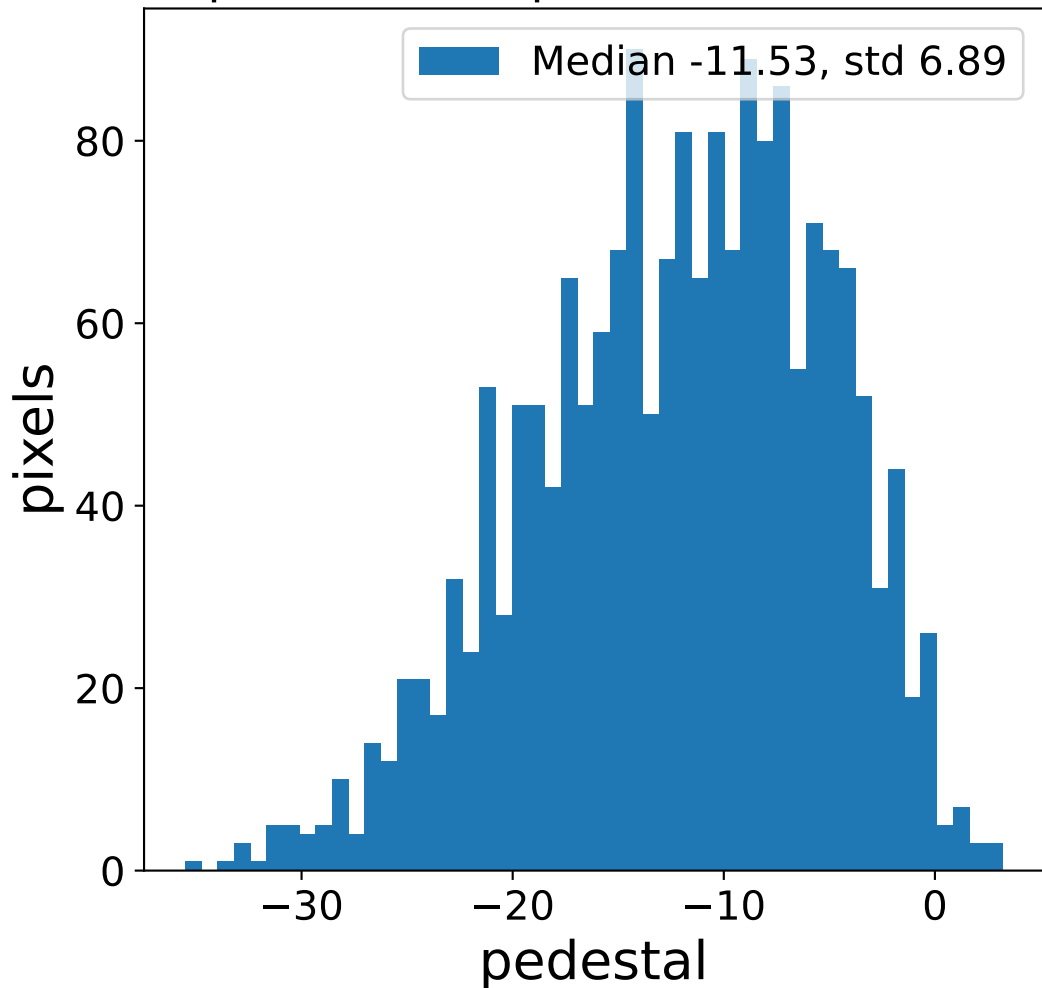
pedestal sample of 2781 events
