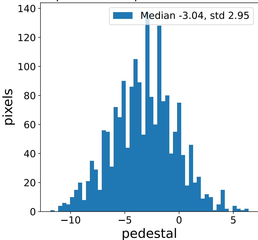
pedestal sample of 2781 events
