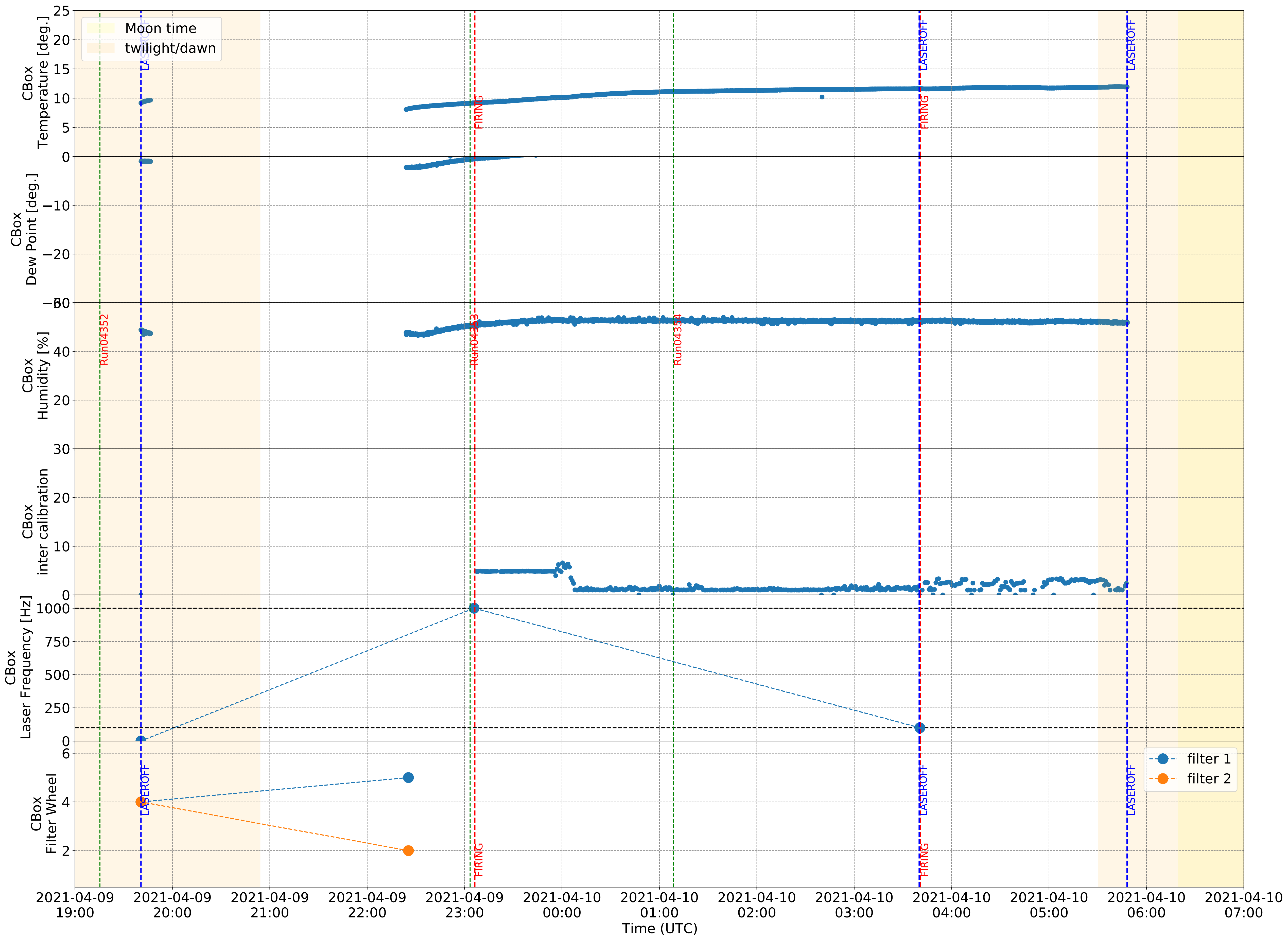
Calibration Box (2021-4-9)
