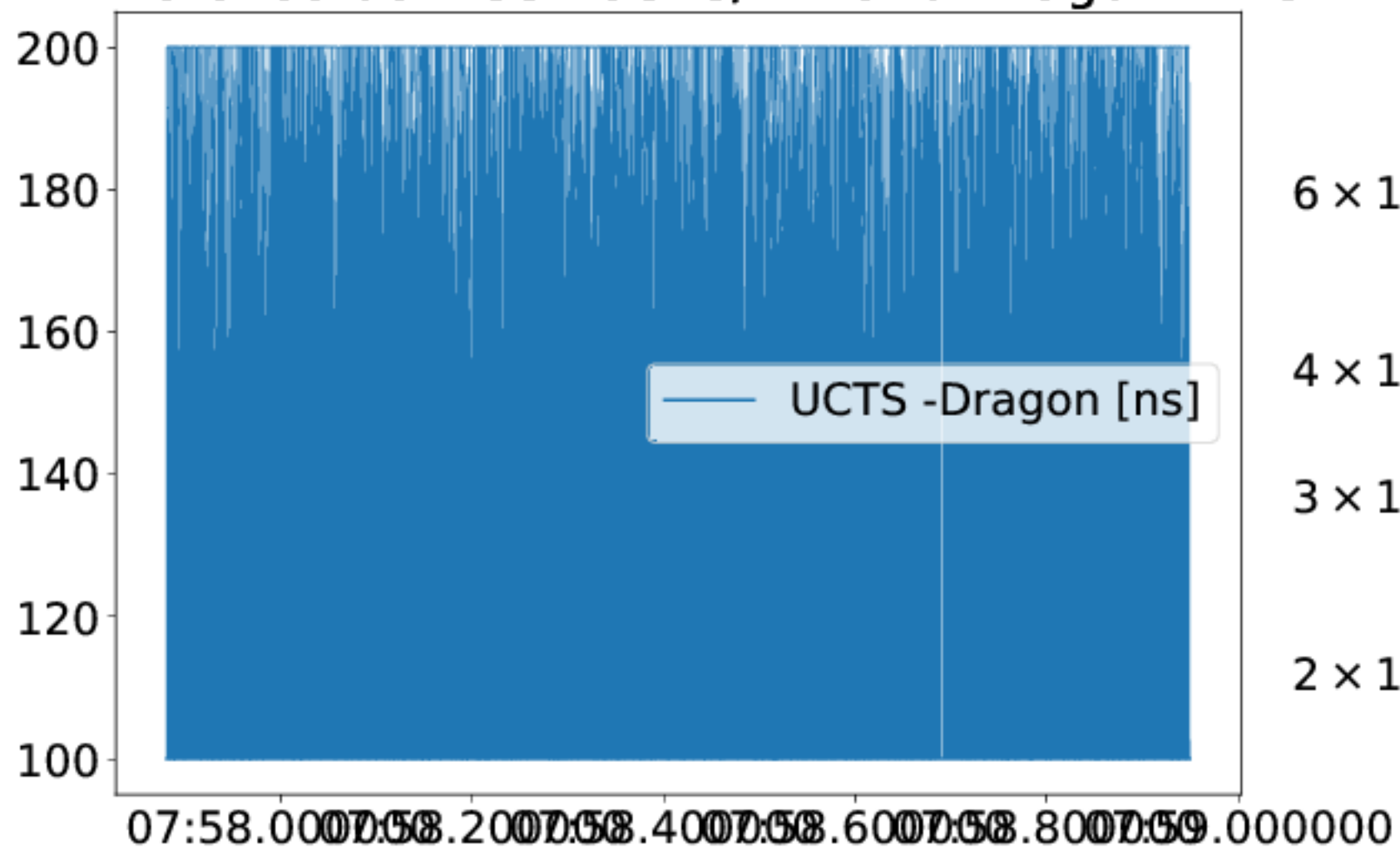
Difference between USTS/TIB and Dragon time
