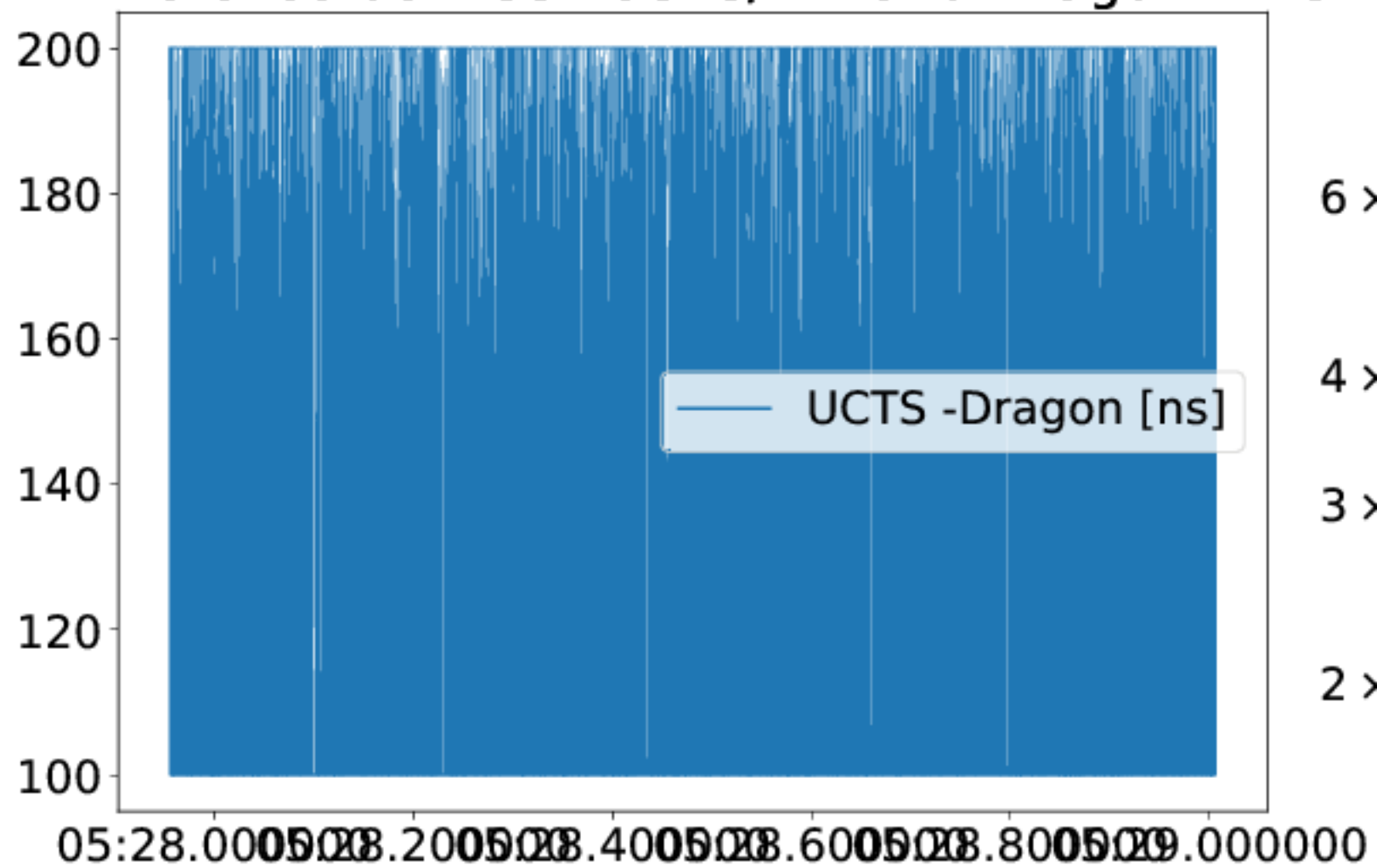
Difference between USTS/TIB and Dragon time
